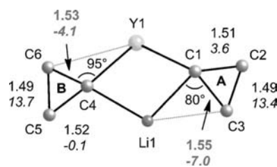
Figure 2. Core of the unsymmetrical optimized structure of 1 with relevant calculated parameters: Top value: CC bond length [Å]; Bottom value (italics): J_{\text{CC}} [Hz].
